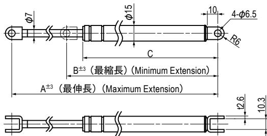
TM-367-50-9・-90-8・-100-8
