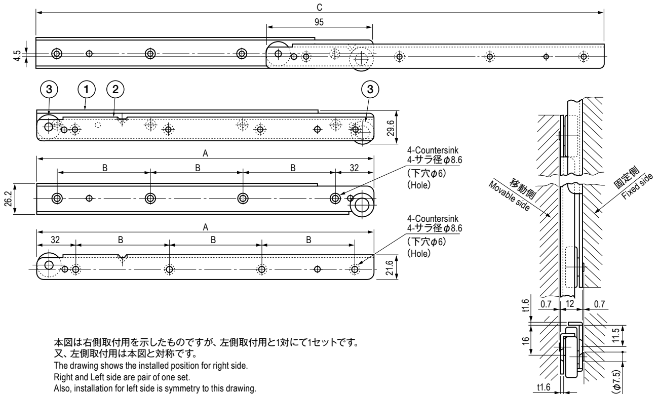
右側取付図 Installation Layout for Right Side
